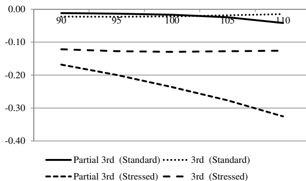
Figure 11: Errors of the partial 3rd and the full 3rd approximations
